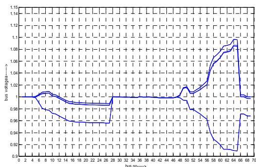
Fig.5 voltage profile for full load with &without DGs connected & voltage control by DGs & Capacitor.
