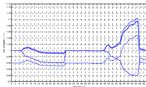
Fig. 9 voltage profile for 90% load with &without DGs connected & voltage control by DGs, Capacitor, and Oltc
