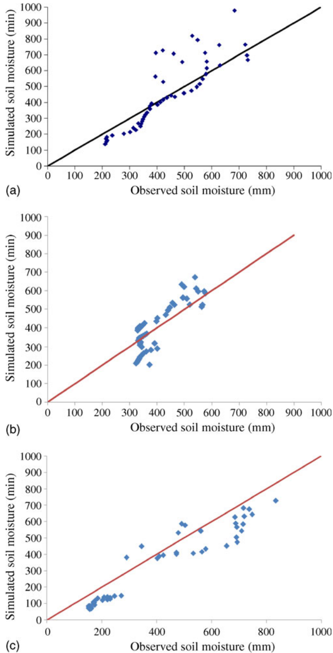
Figure 5. Comparison of observed and simulated soil moisture under different land uses during validation, (a) natural forest, (b) degraded forest, and (c) Acacia .
