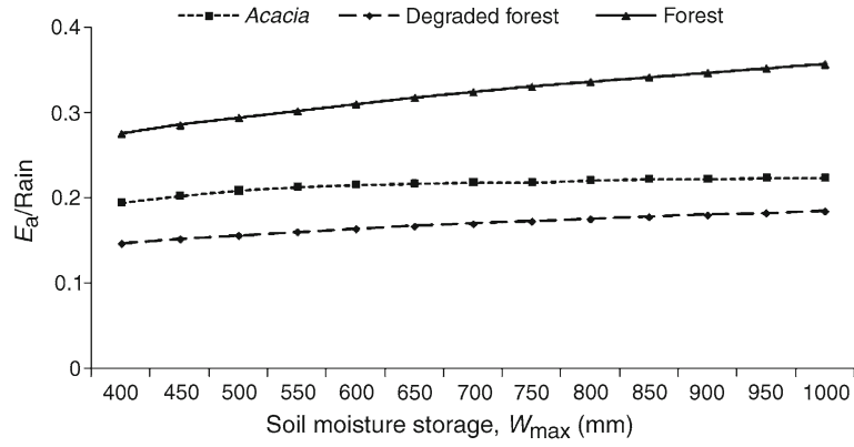
Figure 6. Sensitivity of the mean annual evapotranspiration to changes in soil moisture storage capacity W_{max} . These curves refer to mean annual values scaled by mean annual rainfall. E_a is based on the simulations of 4 years data.
