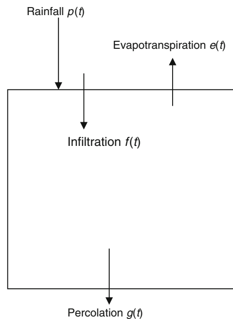
Figure 3. The root zone as a lumped hydrological system.
