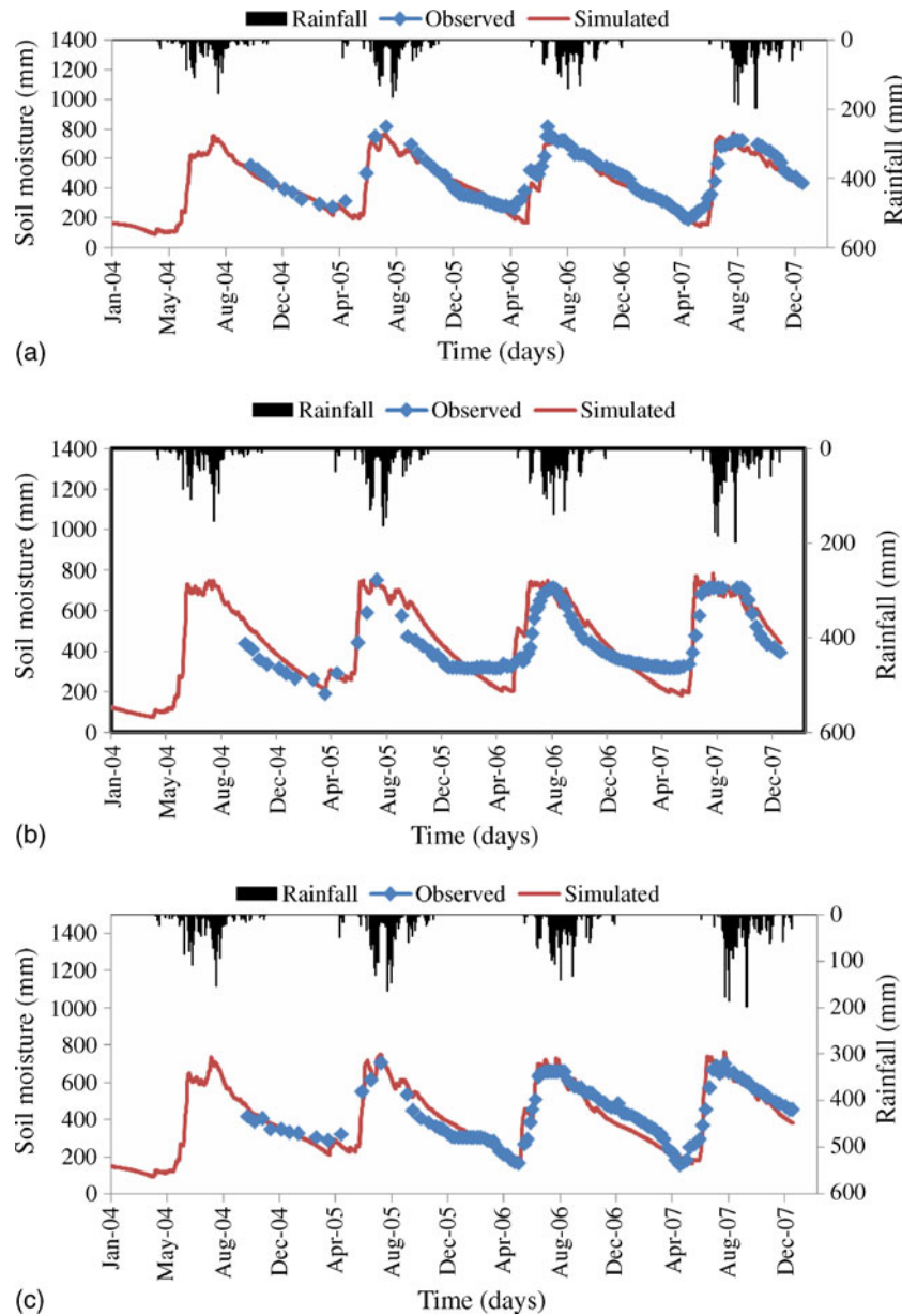
Figure 4. Observed and simulated soil moisture under different land uses during calibration period, (a) natural forest, (b) degraded forest, and (c) Acacia .
