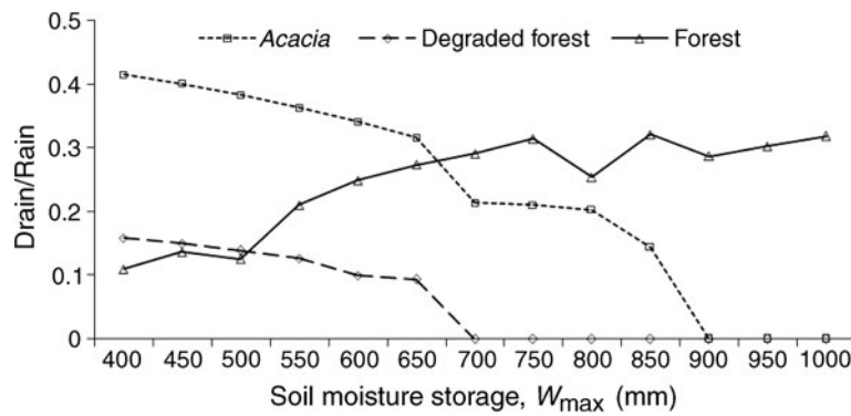
Figure 7. Sensitivity of the mean drainage values to changes in soil moisture storage capacity W_{max} . These curves refer to mean annual values scaled by mean annual rainfall. E_a is based on the simulations of 4-years data.
