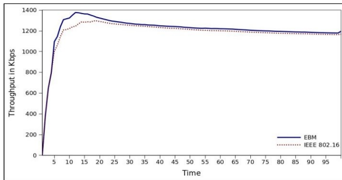
Figure 3. Throughput for rtPS class
