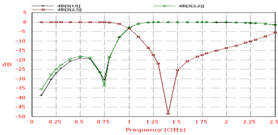
Fig.9. Response of Fractal microstrip Elliptical low pass filter
