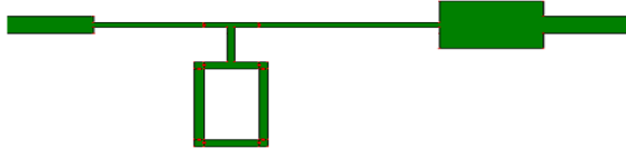
Fig.8. Fractal microstrip Elliptical low pass filter (fractal size 12x6)
