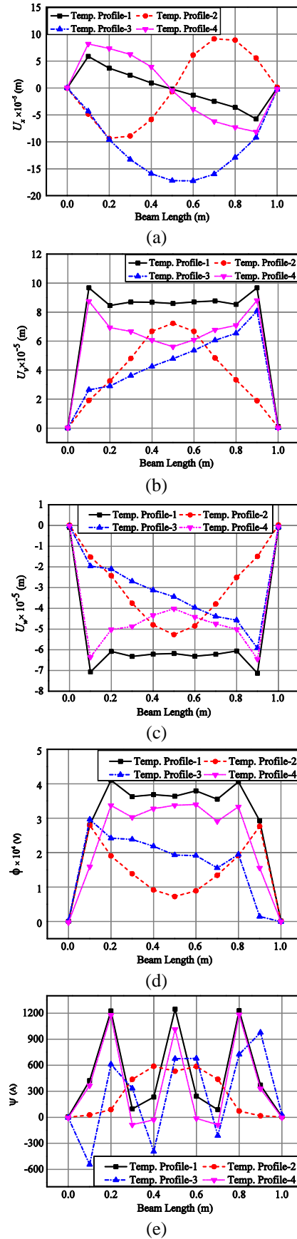
Fig. 8 Variation of (a) longitudinal x -direction ( U_x ) (b) y -direction ( U_y ) (c) z -direction ( U_w ) displacement components (d) electric potential ( \phi ) (e) magnetic potential ( \psi ) for various temperature profiles for C-C boundary condition
