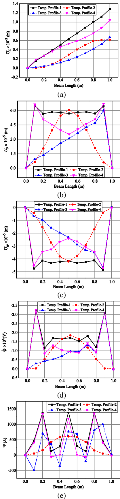
Fig. 9 Variation of (a) longitudinal x -direction ( U_x ) (b) y -direction ( U_y ) (c) z -direction displacement components ( U_z ) (d) electric potential ( \phi ) (e) magnetic potential ( \psi ) for various temperature profiles for C-S boundary condition
