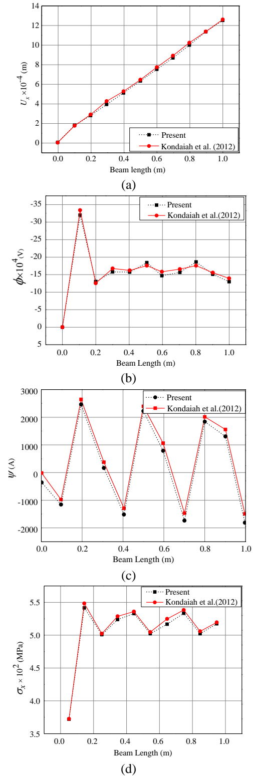
Fig. 2 Validation of (a) longitudinal x -direction ( U_x ) (b) electric potential ( \phi ) (c) magnetic potential ( \psi ) (d) normal stress- \sigma_x
